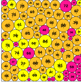
N = 86 86 circles in a square
