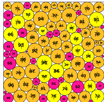
N = 96 96 circles in a square
