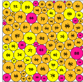
N = 90 90 circles in a square
