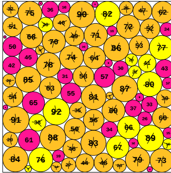
N = 92 92 circles in a square
