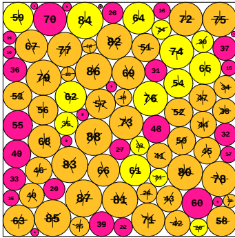
N = 88 88 circles in a square
