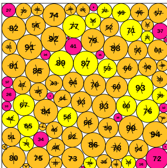
N = 94 94 circles in a square
