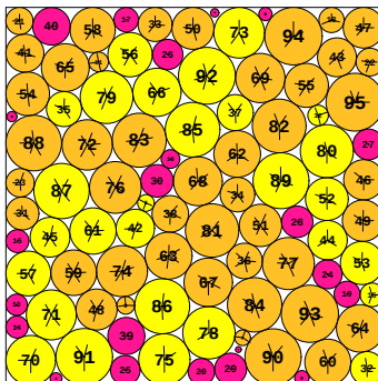
N = 95 95 circles in a square
