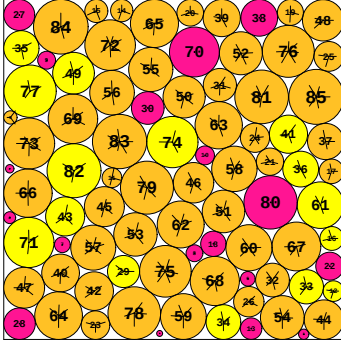
N = 85 85 circles in a square
