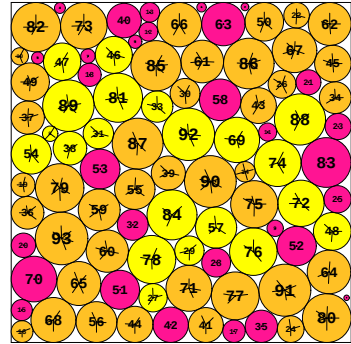
N = 93 93 circles in a square
