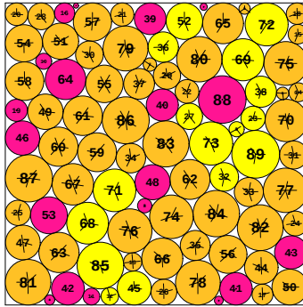
N = 89 89 circles in a square
