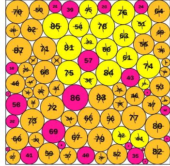
N = 87 87 circles in a square
