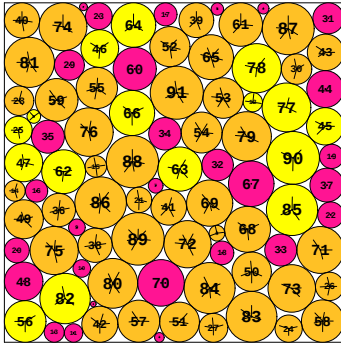
N = 91 91 circles in a square
