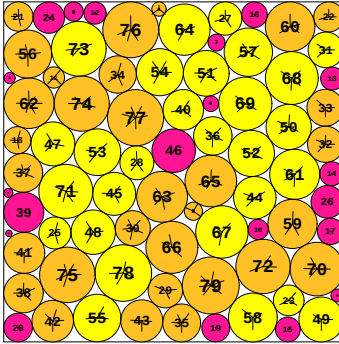
N = 79 79 circles in a square
