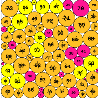
N = 73 73 circles in a square
