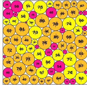
N = 81 81 circles in a square
