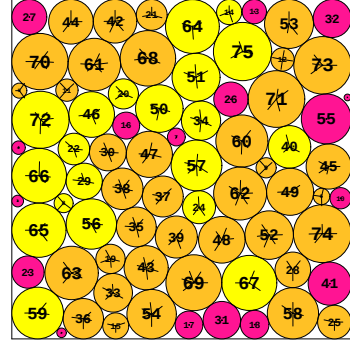
N = 75 75 circles in a square
