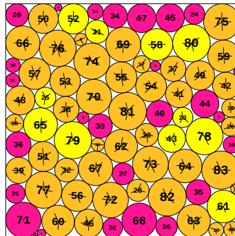
N = 83 83 circles in a square
