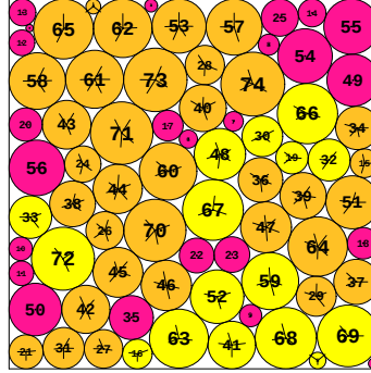
N = 74 74 circles in a square
