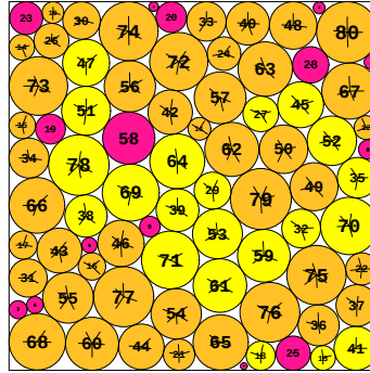
N = 80 80 circles in a square
