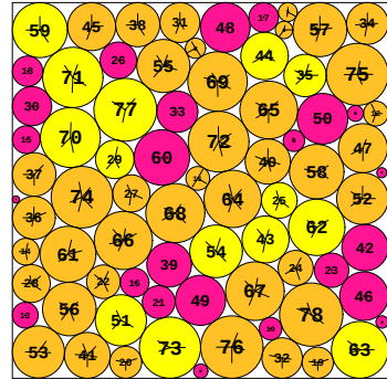
N = 78 78 circles in a square
