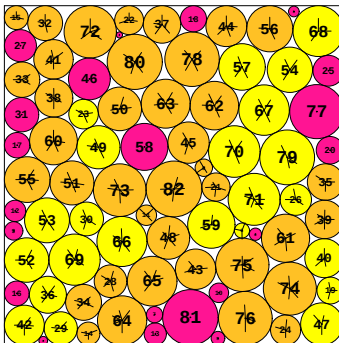
N = 82 82 circles in a square
