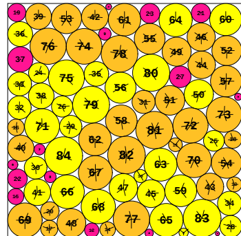
N = 84 84 circles in a square
