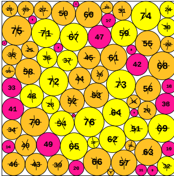
N = 76 76 circles in a square
