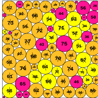
N = 77 77 circles in a square
