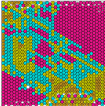
N = 1224 1224 circles in a square
