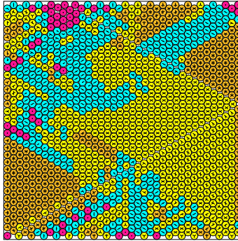
N = 1216 1216 circles in a square
