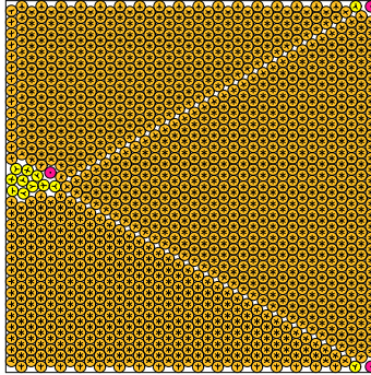
N = 1198 1198 circles in a square
