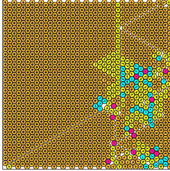
N = 1190 1190 circles in a square
