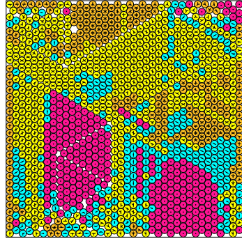
N = 1206 1206 circles in a square
