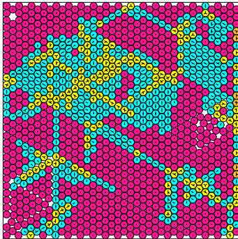
N = 1221 1221 circles in a square
