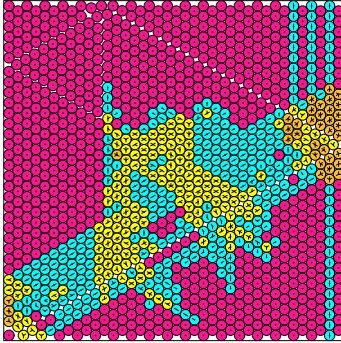
N = 1197 1197 circles in a square
