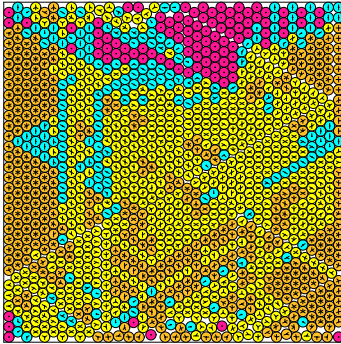
N = 1209 1209 circles in a square
