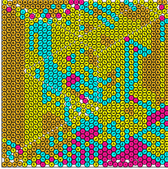
N = 1188 1188 circles in a square
