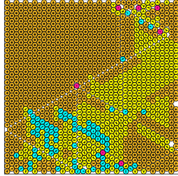
N = 1191 1191 circles in a square
