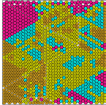
N = 1220 1220 circles in a square
