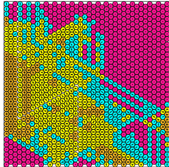
N = 1229 1229 circles in a square
