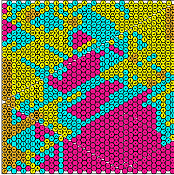
N = 1147 1147 circles in a square
