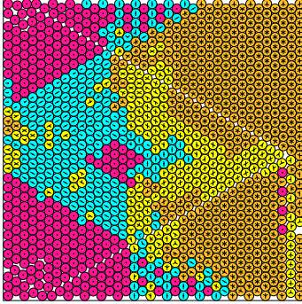
N = 1130 1130 circles in a square
