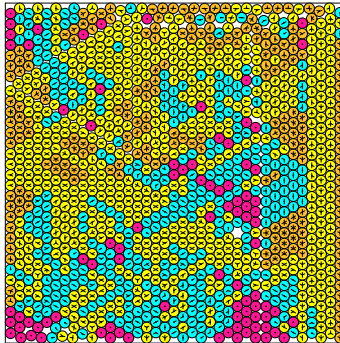
N = 1170 1170 circles in a square
