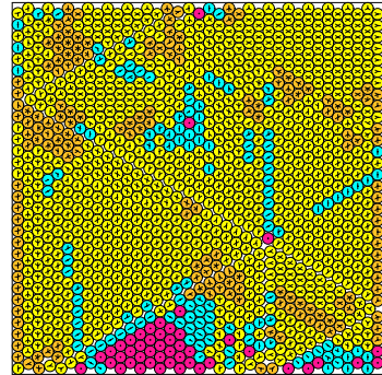
N = 1178 1178 circles in a square
