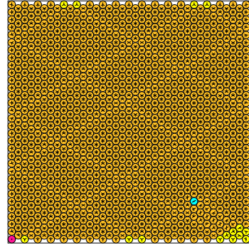
N = 1166 1166 circles in a square
