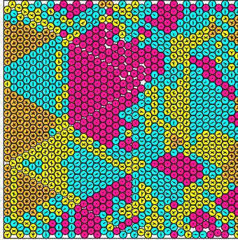
N = 1151 1151 circles in a square
