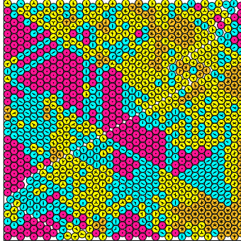
N = 1134 1134 circles in a square
