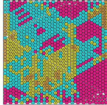
N = 1152 1152 circles in a square
