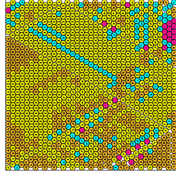
N = 1140 1140 circles in a square
