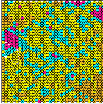
N = 1160 1160 circles in a square
