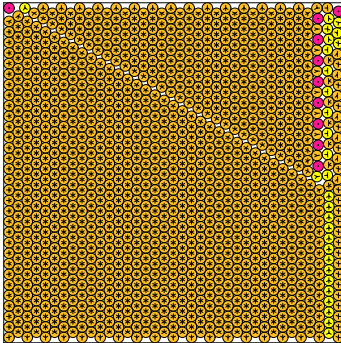
N = 1167 1167 circles in a square
