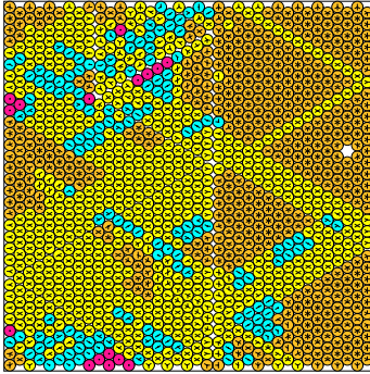
N = 1159 1159 circles in a square
