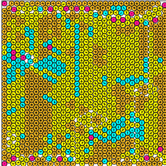
N = 1105 1105 circles in a square
