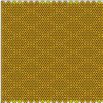
N = 1098 1098 circles in a square
