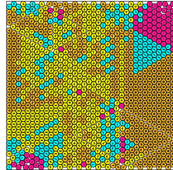
N = 1102 1102 circles in a square
