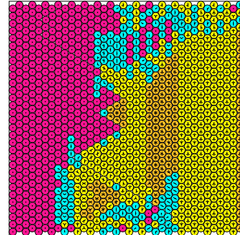
N = 1116 1116 circles in a square
