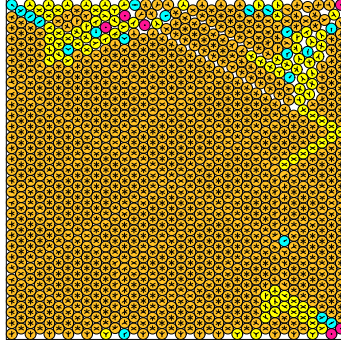
N = 1092 1092 circles in a square
