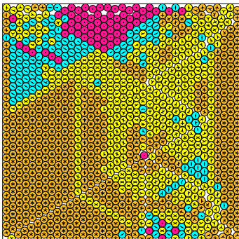
N = 1121 1121 circles in a square
