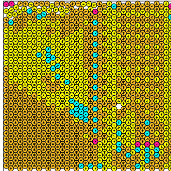
N = 1110 1110 circles in a square
