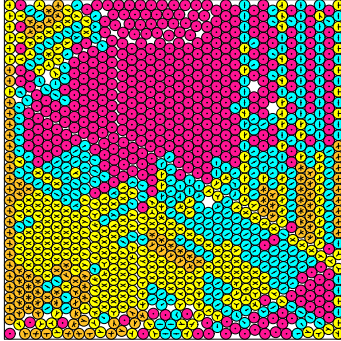
N = 1088 1088 circles in a square
