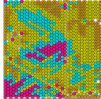
N = 1093 1093 circles in a square
