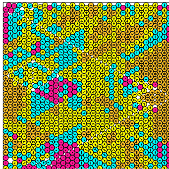
N = 1122 1122 circles in a square
