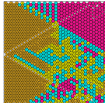
N = 1129 1129 circles in a square
