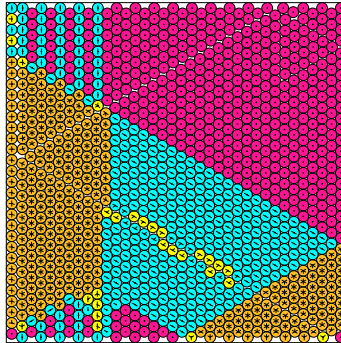
N = 1099 1099 circles in a square
